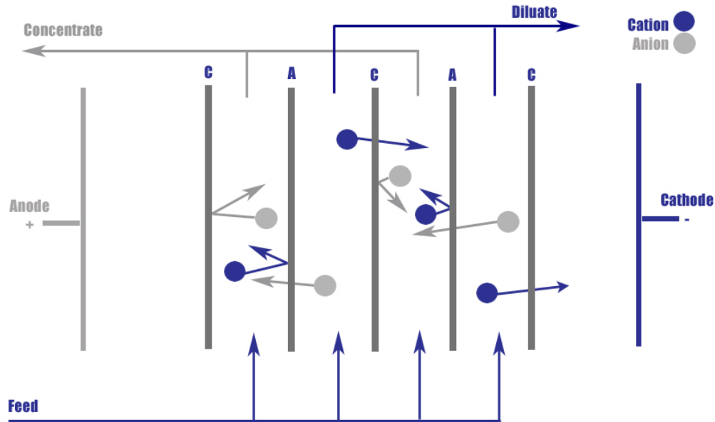
Figure 4: Electrodialysis system
